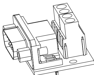
ADP-090401 adapter changing 4 into 9 PIN (special between 232, 485 and 422, order separately)
